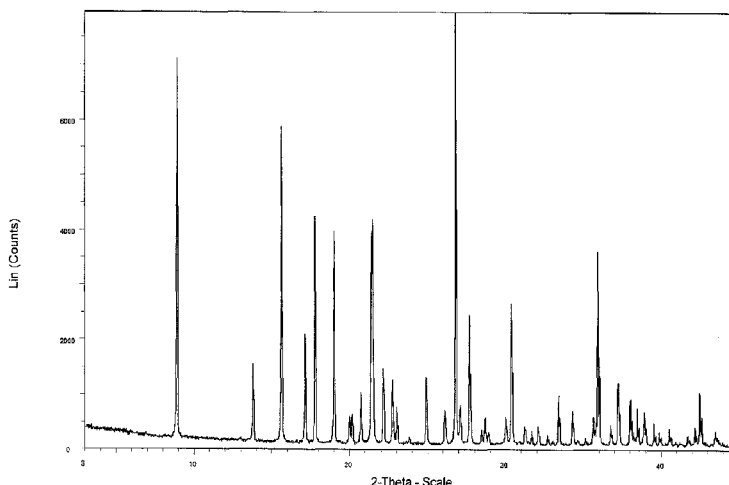
PXRD pattern of potassium 2,5-dihydroxybenzenesulfonic acid (Example 6)
